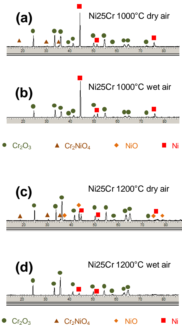
Figure 3 : Examples of results of x-ray diffraction performed on the surfaces of the oxidized Ni25Cr samples: after oxidation at 1000°C in dry (a) or wet (b) air, and after oxidation at 1200°C in dry (c) or wet (d) air
