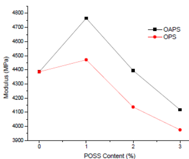
FIG. 5. Effect of POSS content on modulus.
